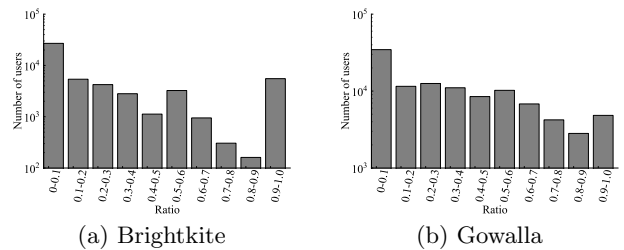
Figure 4: Distribution of users according to the impact of the community in the places they choose to visit.
