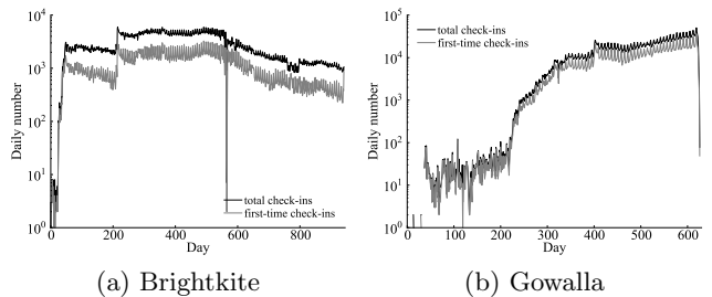
Figure 1: Daily number of check-in records in Brightkite and Gowalla.
